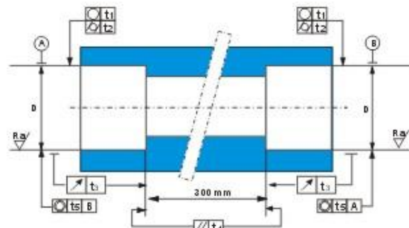
配合轴和座 Fitting shaft and housing
