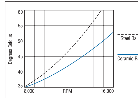
Lower operating temperature. As running speeds increase, ceramic balls always run cooler than conventional steel balls. With reduced heat build up, lubricant life is prolonged.
