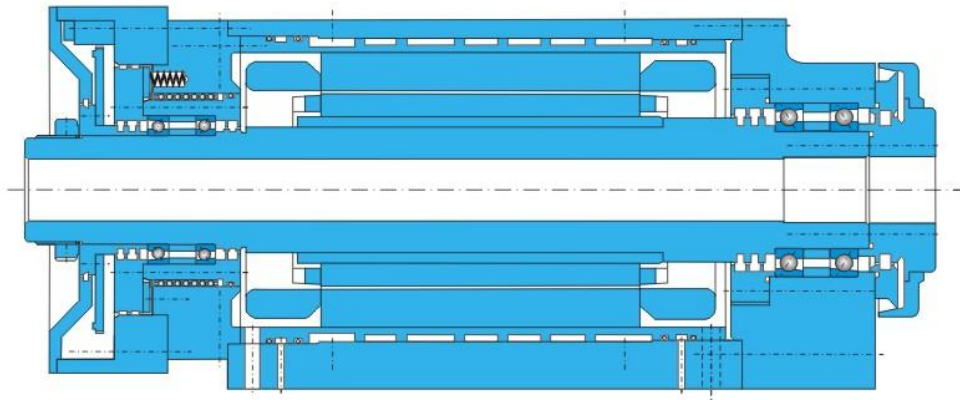
Fig. 34 Spindle for high-speed milling machine
