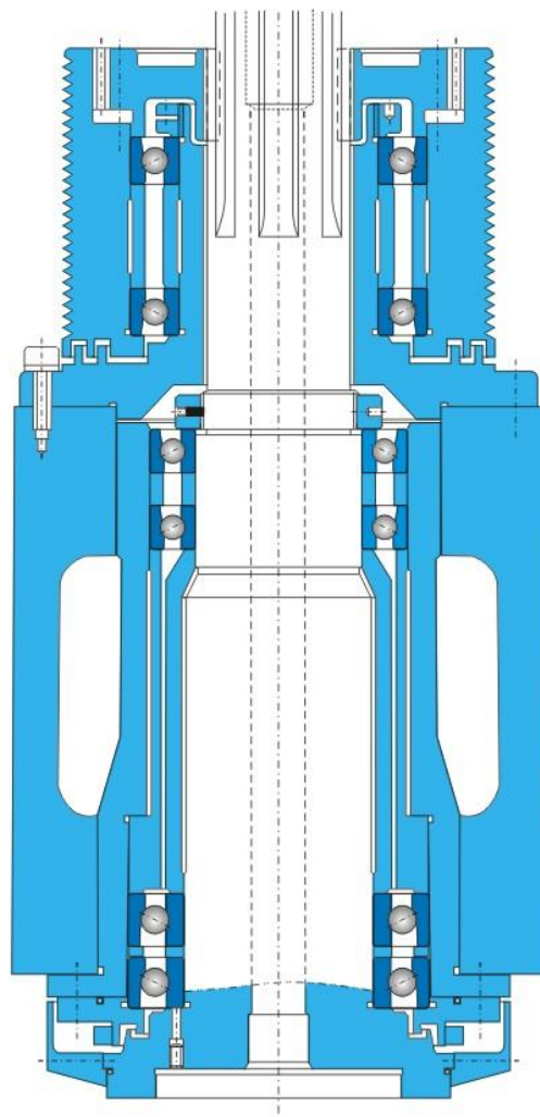
Fig. 24 Super-speed CNC lathe spindle
