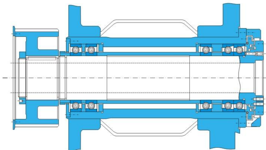
Fig. 37 Spindle for machining center
