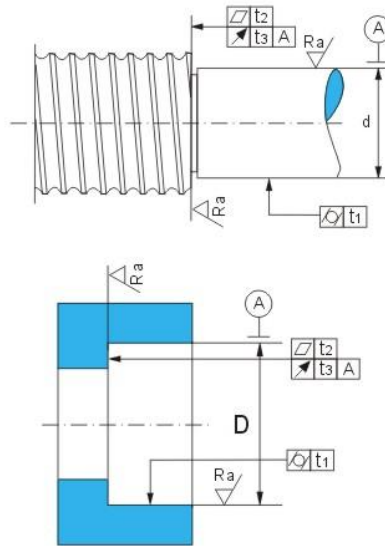
Fig. 17 Fitting parts for ball screw support bearings
