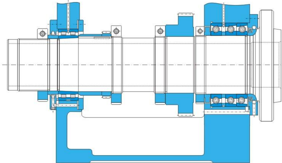
Fig. 27 High rigidity lathe spindle
