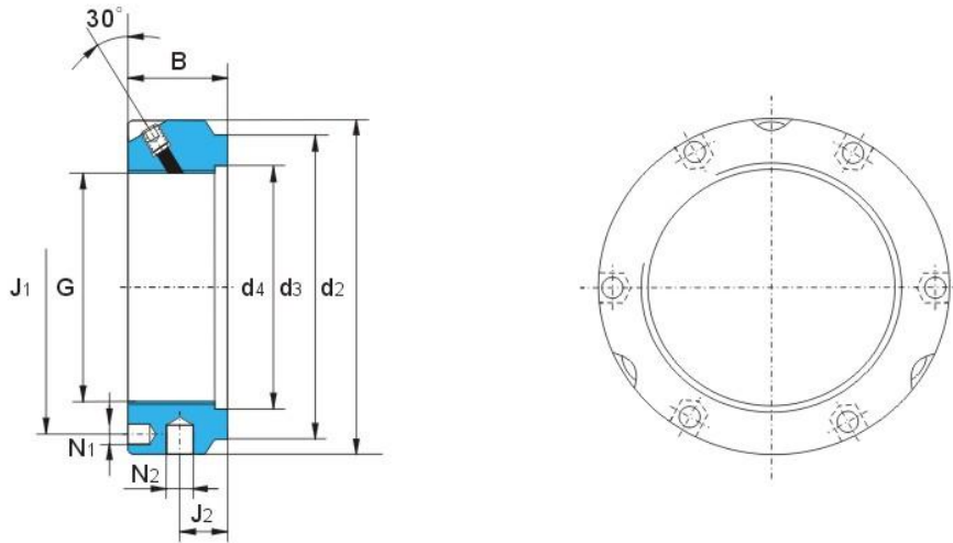
KMB-type locknuts
