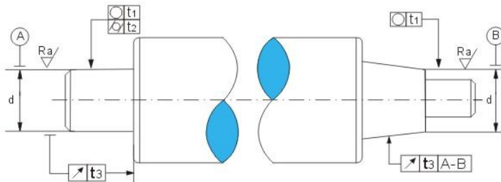
Fig. 16 Fitting tapered shaft
