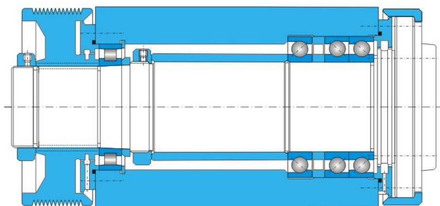
Fig. 38 Spindle for turning center
