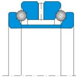
Fig. 3 ZYS Double-direction angular contact thrust ball bearings
