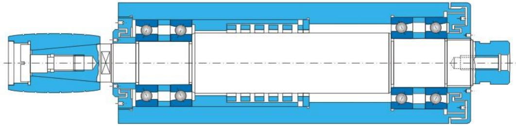
Fig. 29 Spindle for bore diameter grinding machine
