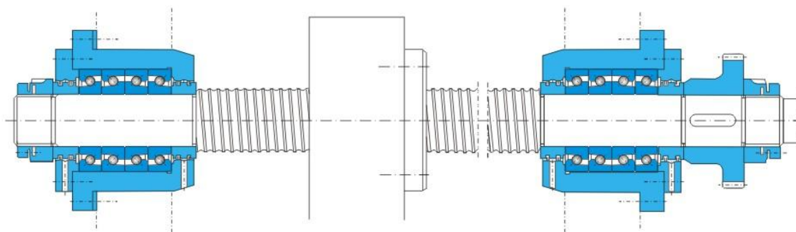
Fig. 39 Ball screw support
