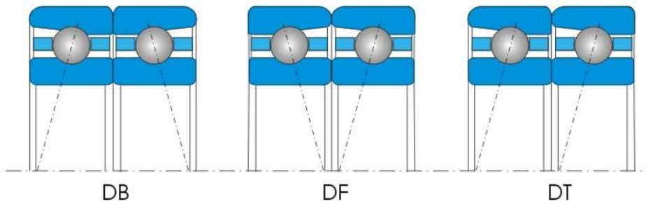
Fig. 18 Structures of duplex configuration bearings
