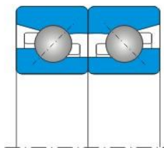
Fig. 4 High-speed angular contact thrust ball bearing structure
