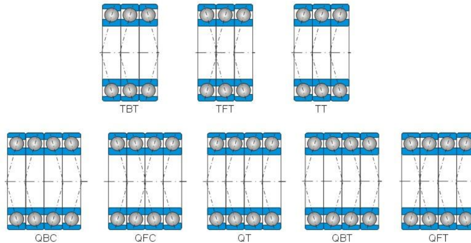
Fig. 19 Multiple arrangement bearings
