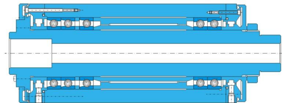
Fig. 36 Spindle for drilling machine
