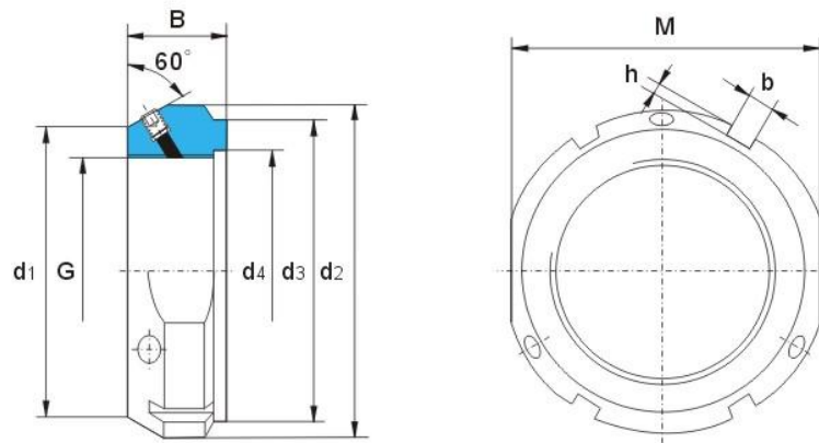
KMA-type locknuts
