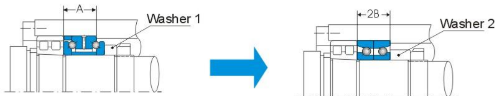
Fig. 5 The mounting of high-speed angular contact thrust ball bearings
