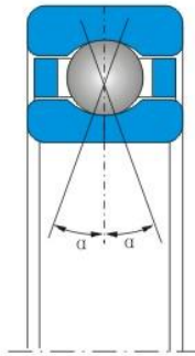
Fig. 11 Four-point contact ball bearings for turbo charger
